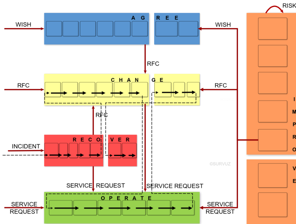
Figure 5. USM workflows are predefined logical sequences of activities in the USM process model
